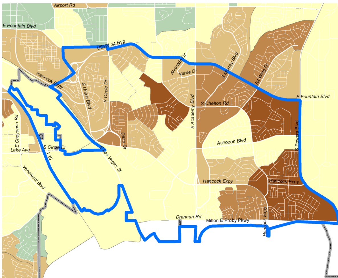
Figure 87: Urban heat Island Effect
