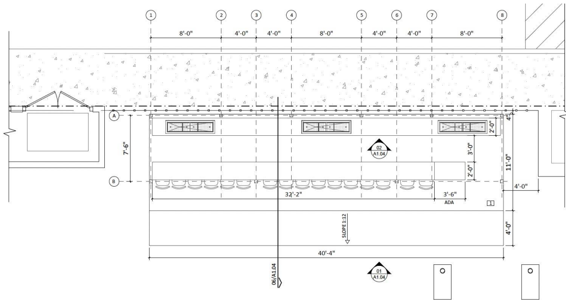
Construction Floor Plan
