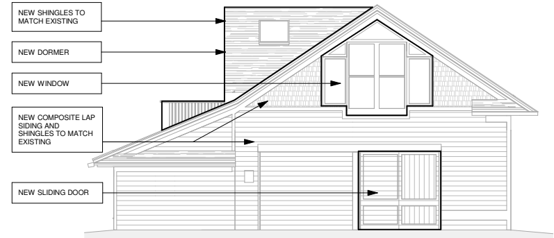
4 2 Proposed West View 1/8" = 1'-0"
