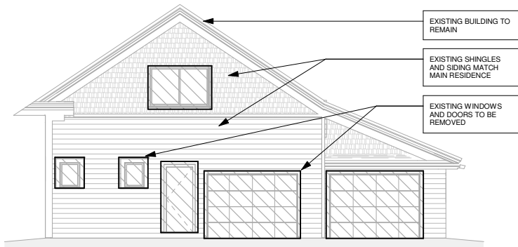
1 1 Existing East View 1/8" = 1'-0"
