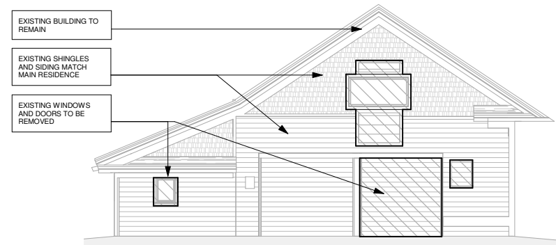
2 1 Existing West View 1/8" = 1'-0"
