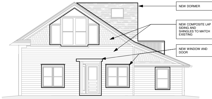
3 2 Proposed East View 1/8" = 1'-0"
