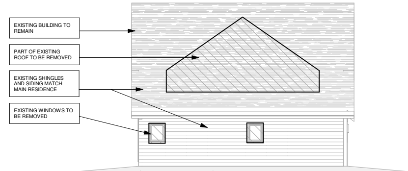
2 1 Existing North View 1/8" = 1'-0"
