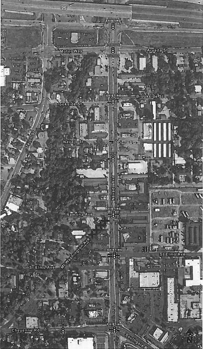
Exhibit A: Proposed South Nevada Signalization Plan per City Traffic
