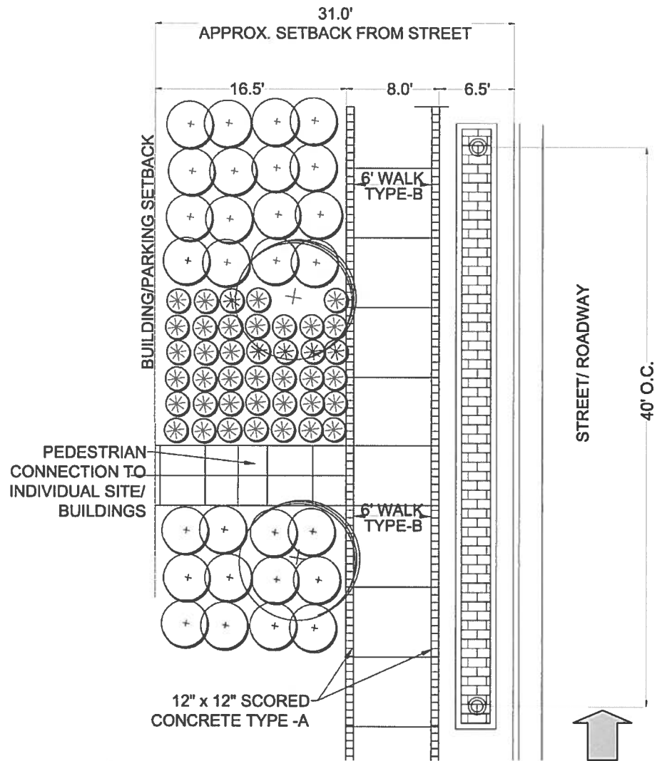
Cheyenne Road, North Side Section and Plan
