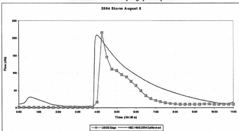
Figure III-4 2004 Storm – Calibrated Hydrograph Comparison
