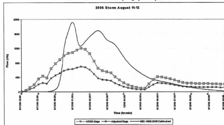
Figure III-6 2006 Storm – Calibrated Hydrograph Comparison
