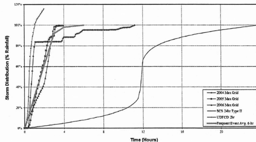
Figure III-1 2004, 2005, 2006 Storm Distributions Calibrated NEXRAD Data
