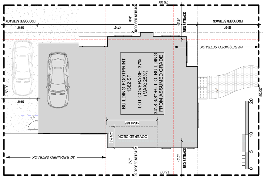
1 SITE PLAN SCALE: 1/8" = 1'-0" - (1/16" ELEV)
