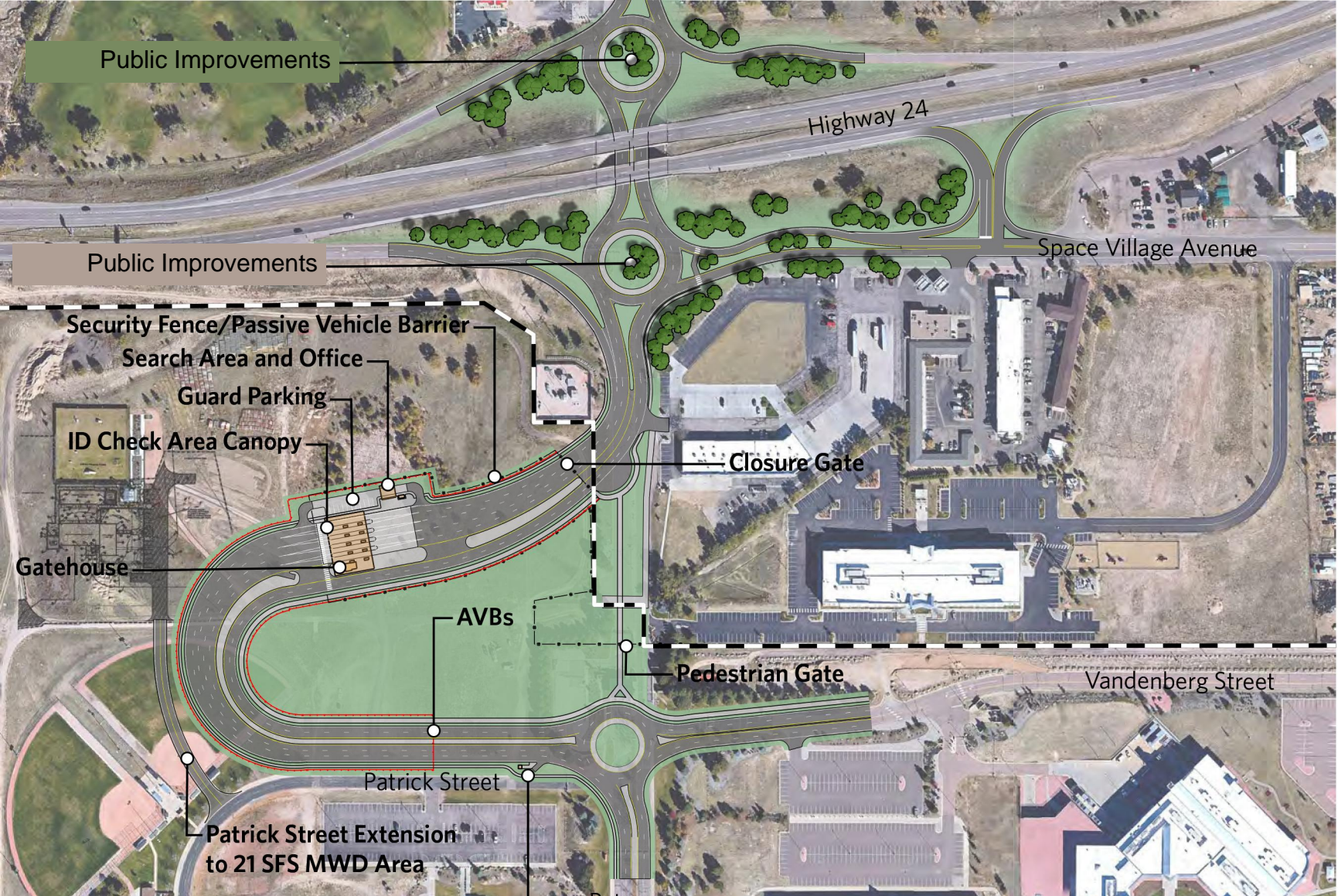
Preliminary PAFB/Highway 24 Interchange Concept
