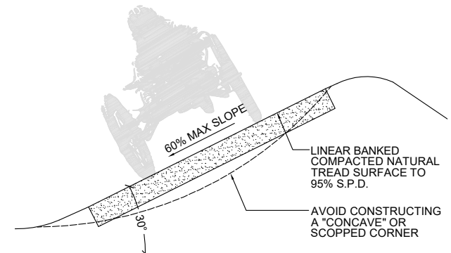
Figure 5 - aMTB Berm
