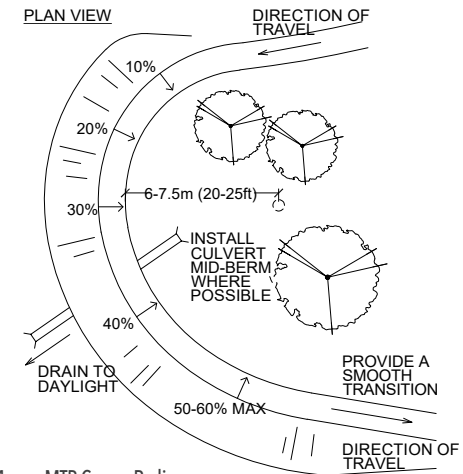
Figure 4 - aMTB Corner Radius
