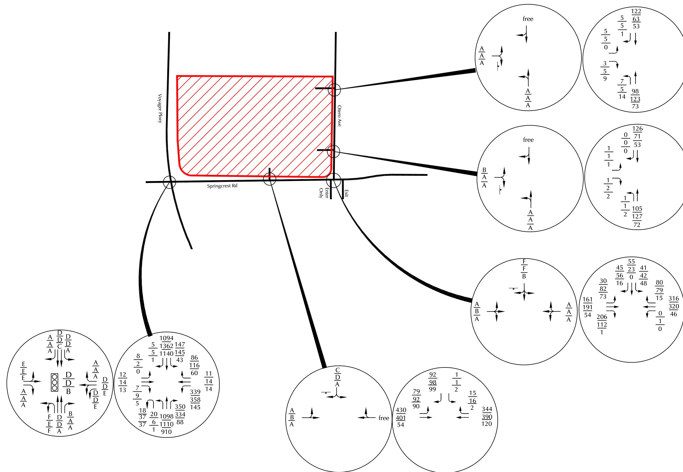
Figure 8 2044 Background + Site-Generated Traffic, Lane Geometry, Traffic Control, and LOS
