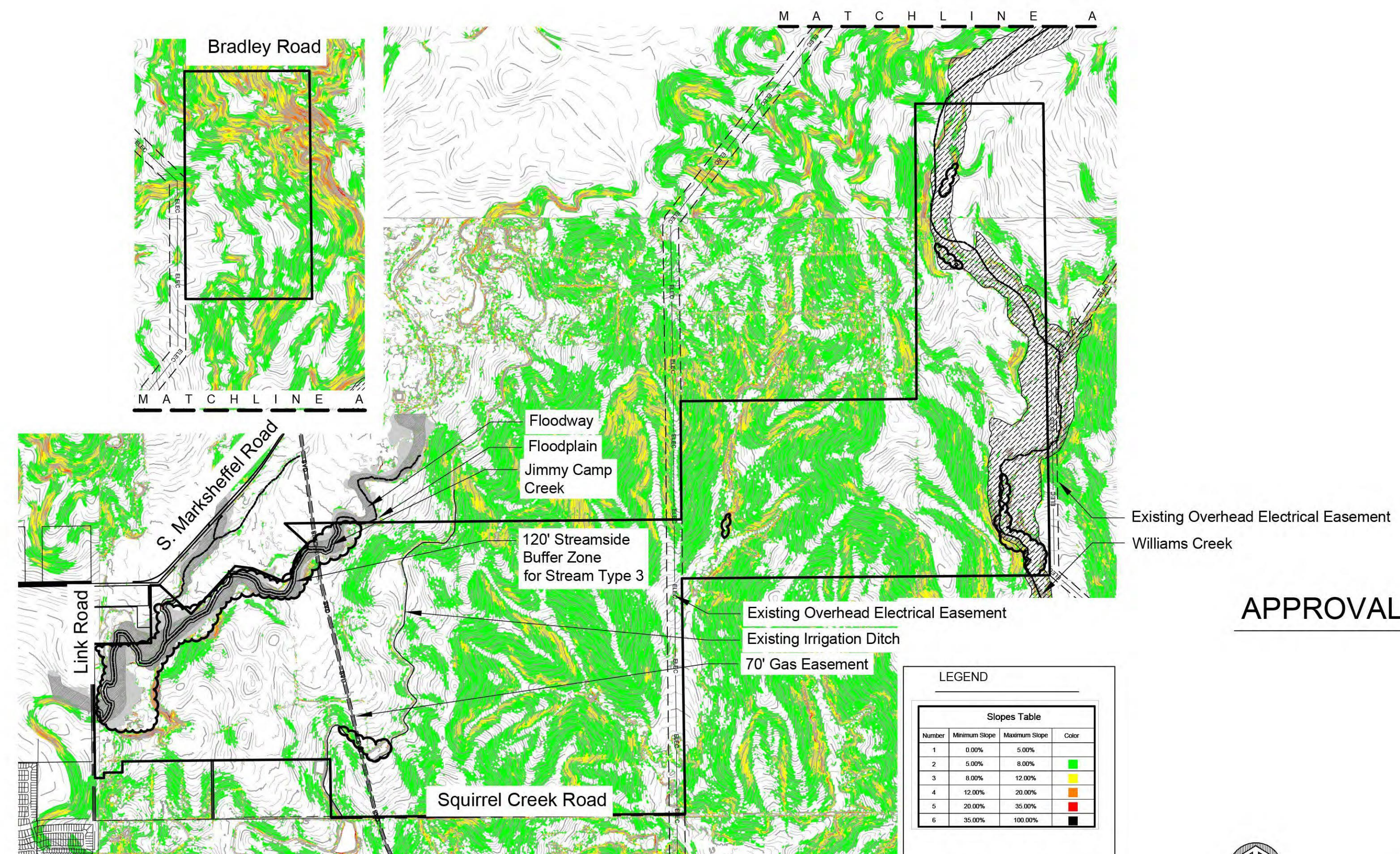
COMPOSITE ANALYSIS
