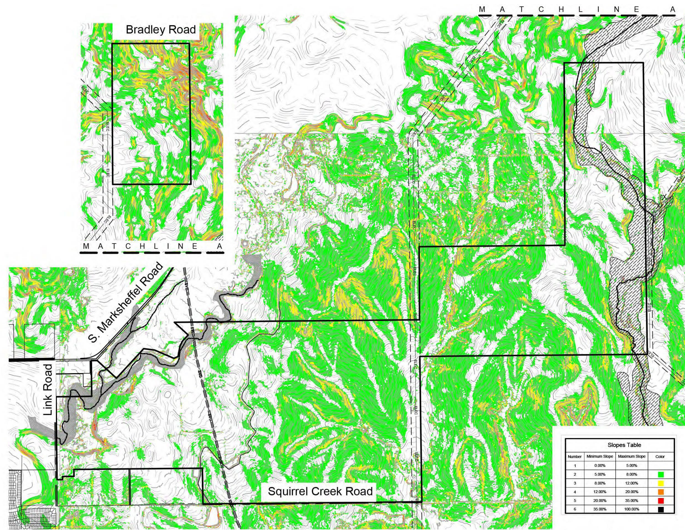
SLOPE ANALYSIS
