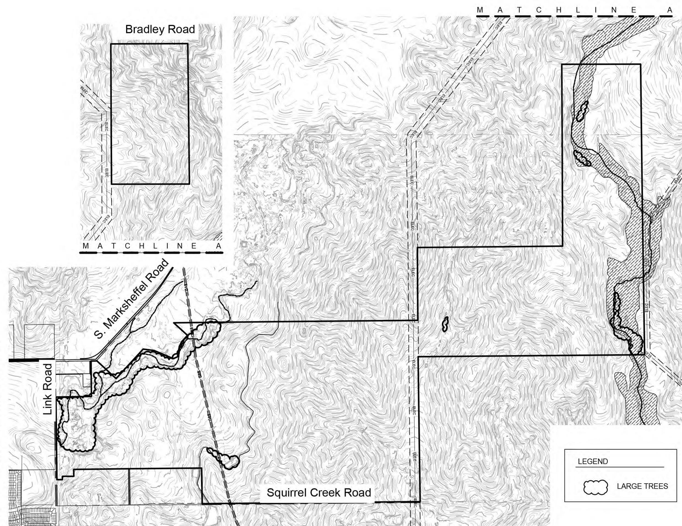
VEGETATION ANALYSIS
