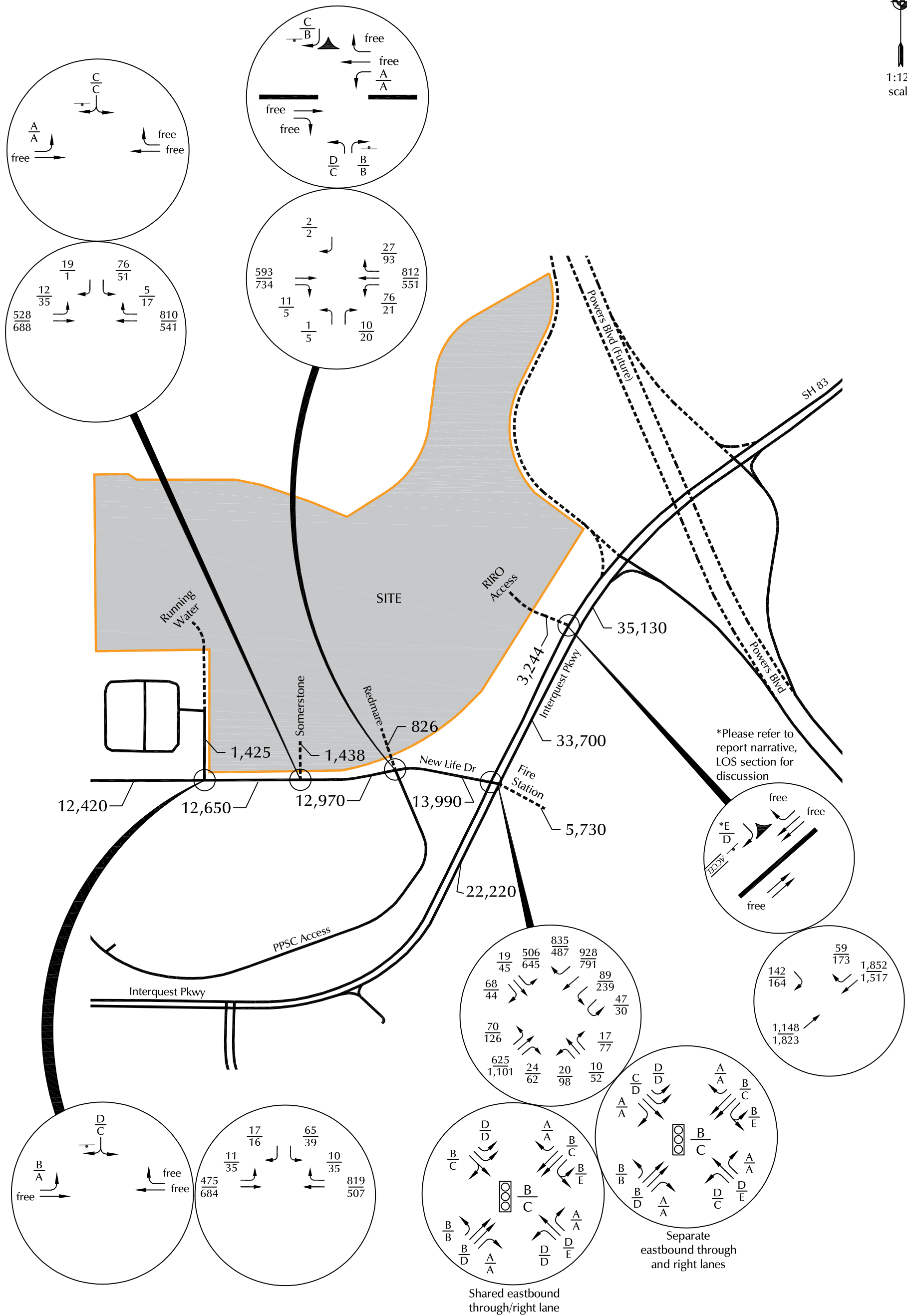
Figure 9 2050 Background + Site Traffic, Lane Geometry, Traffic Control, and LOS Creekridge at Flying Horse (LSC #204611)
