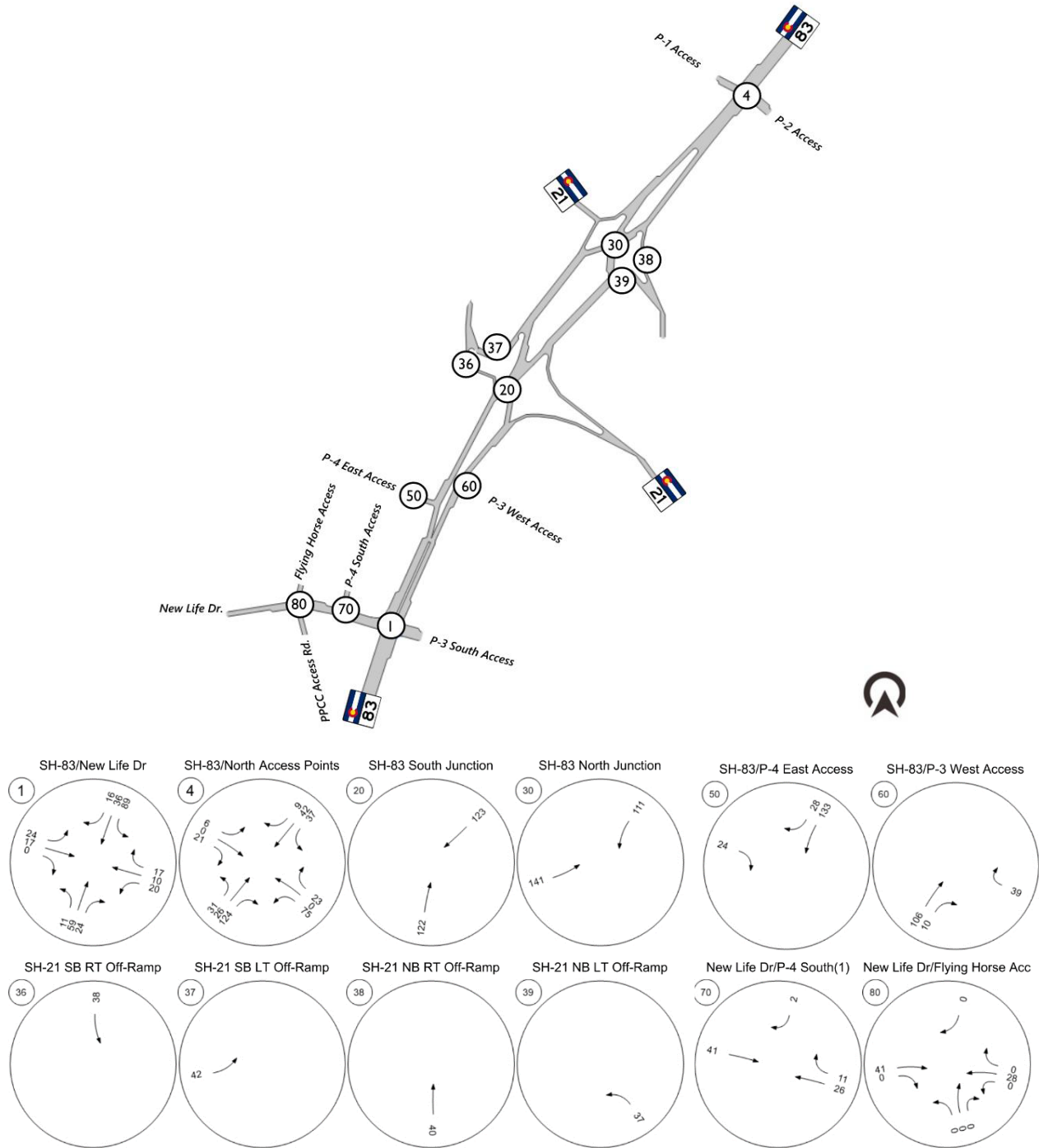
Figure 9. Kettle Creek Center Site Trips (AM Peak Hour)
