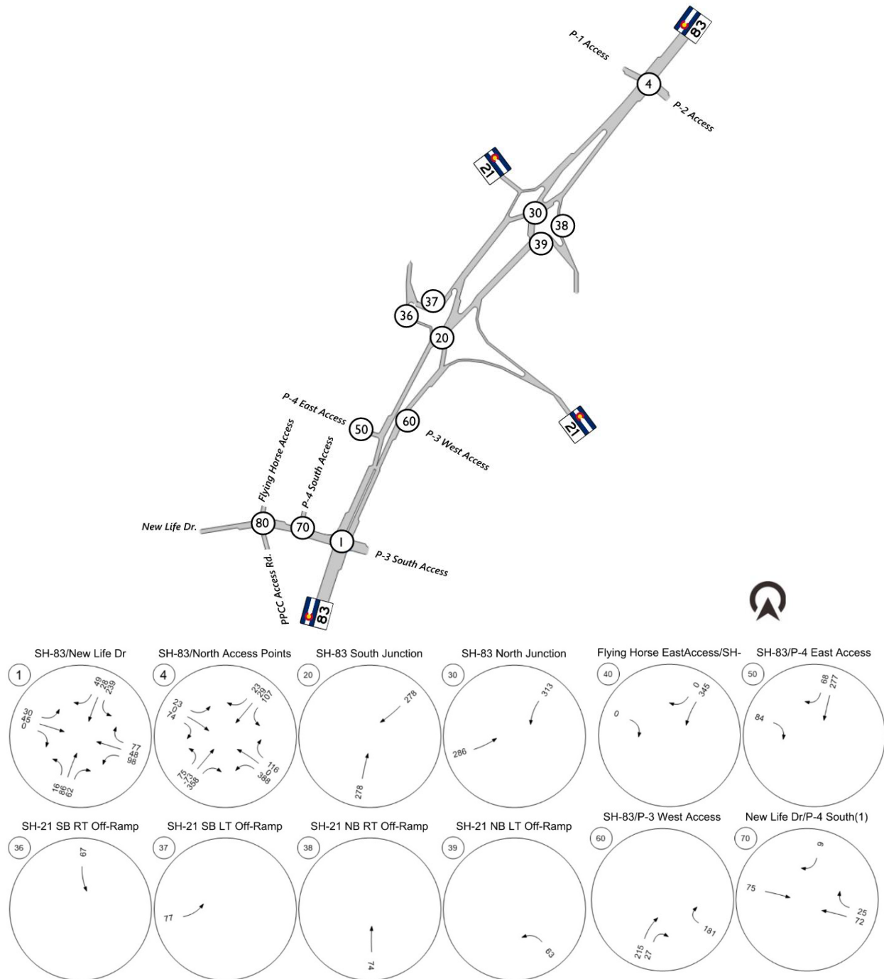
Figure 12. Kettle Creek Center Total Site Trips (PM Peak Hour)
