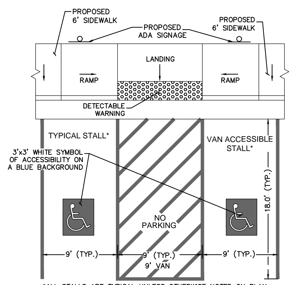
ACCESSIBLE PARKING DETAIL N.T.S.
