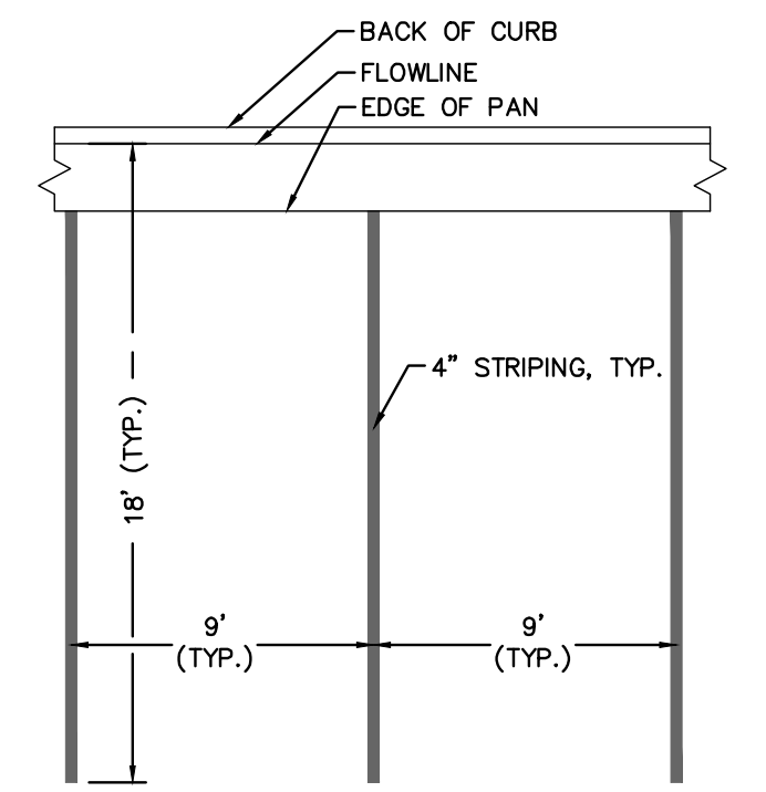
STANDARD PARKING DETAIL N.T.S.
