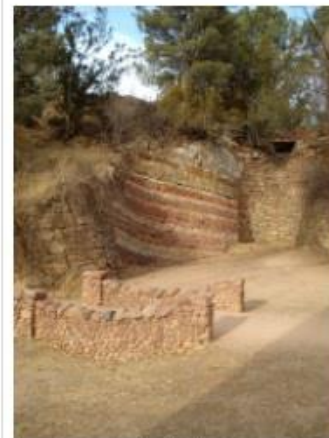
Geologic Column
