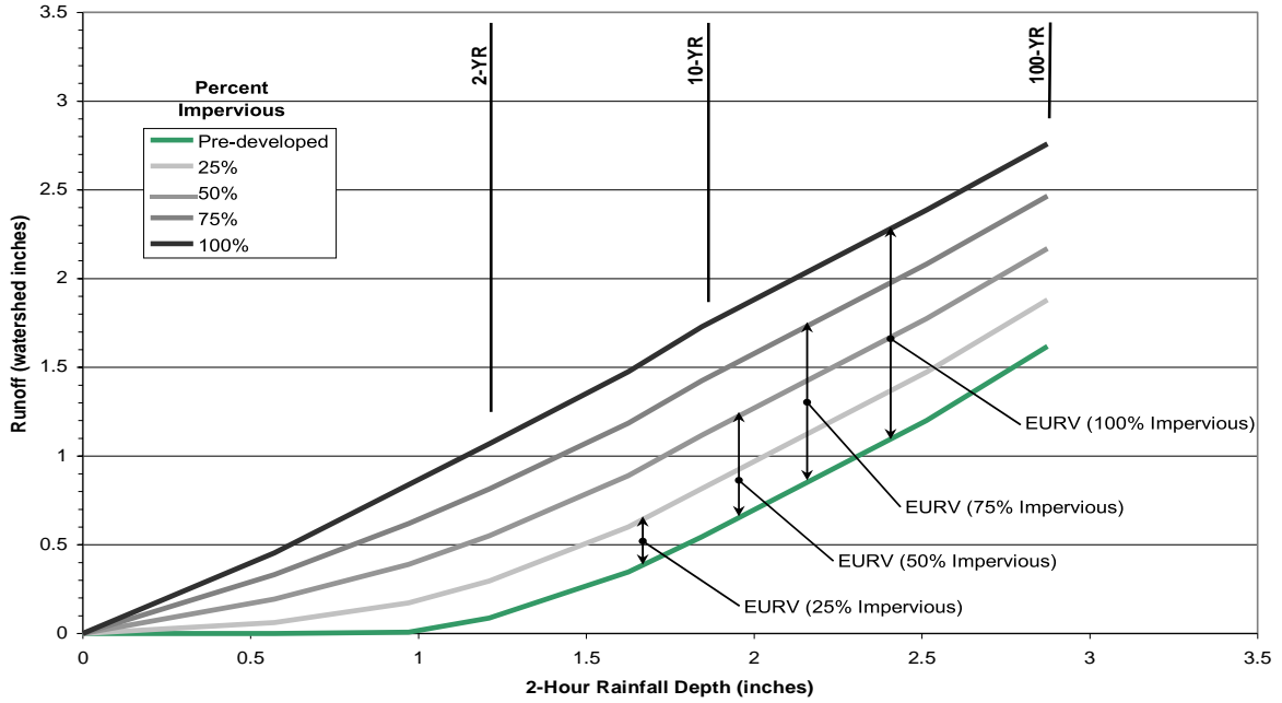
Figure 13-4b. Excess Urban Runoff Volume (EURV) per Impervious Acre [Type C/D Soils]
