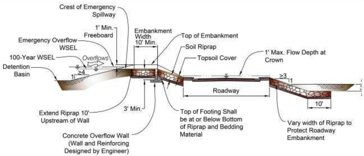
Figure 13-12a. Emergency Spillway Profile at Roadway
