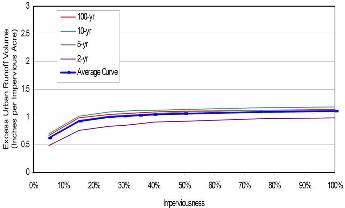
Figure 13-4b. Excess Urban Runoff Volume (EURV) per Impervious Acre [Type C/D Soils]
