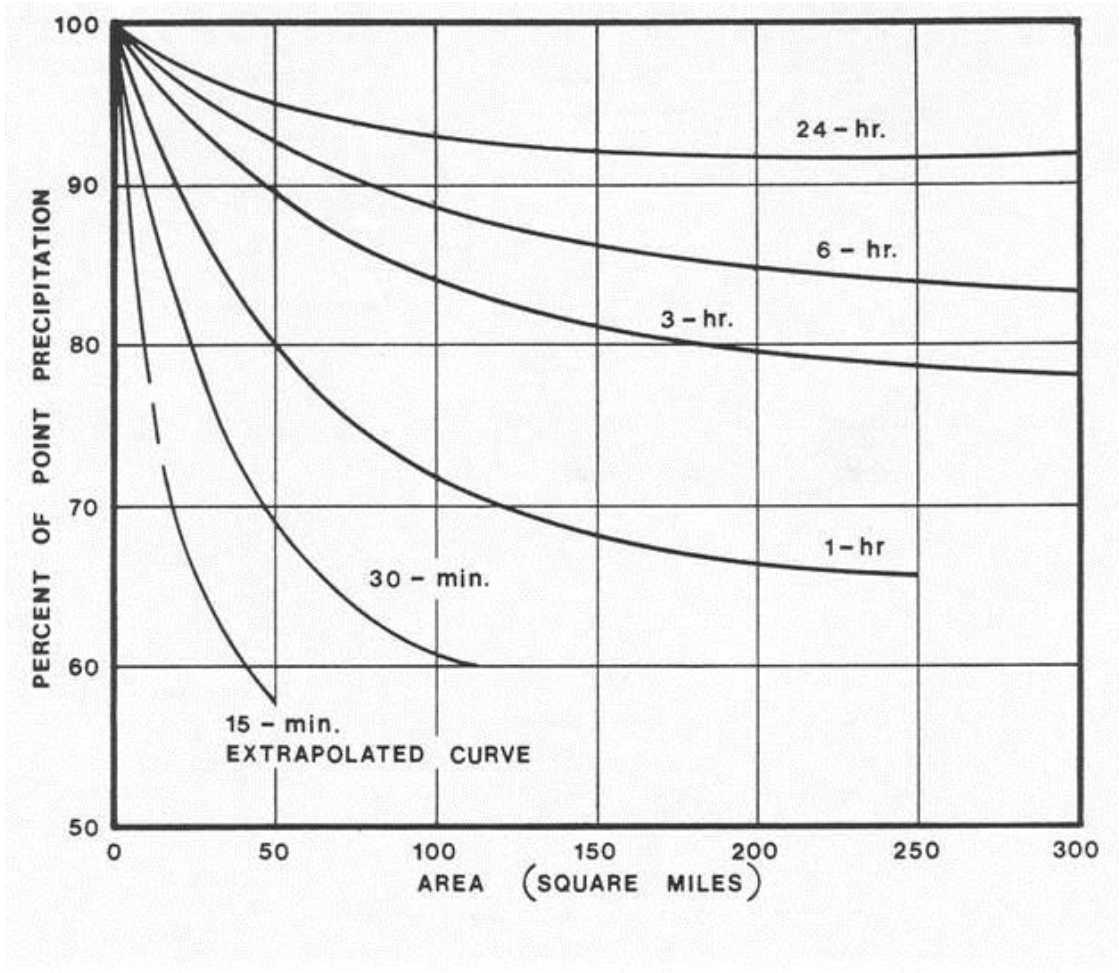
Figure 6-2210. Depth-Area-Duration Adjustment Factors for 24-Hour Frontal Storms
