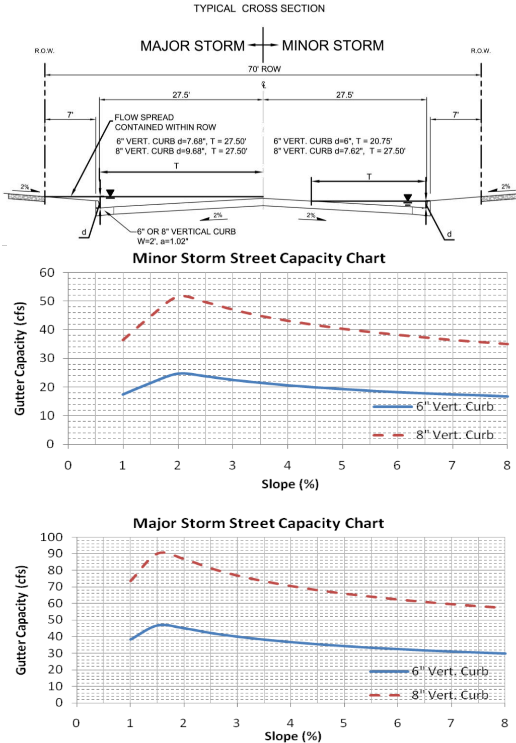
Figure 7-4. Street Capacity Charts Industrial
