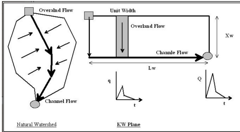
Figure 6-2. Conceptual SWMM Watershed Schematic
