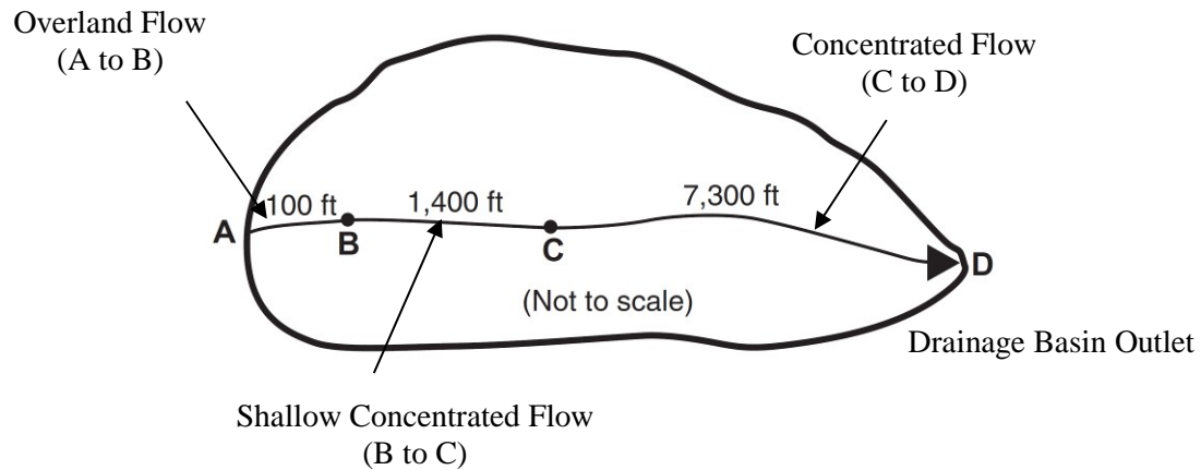
Figure 6-1. Flow Segments for Time of Concentration
