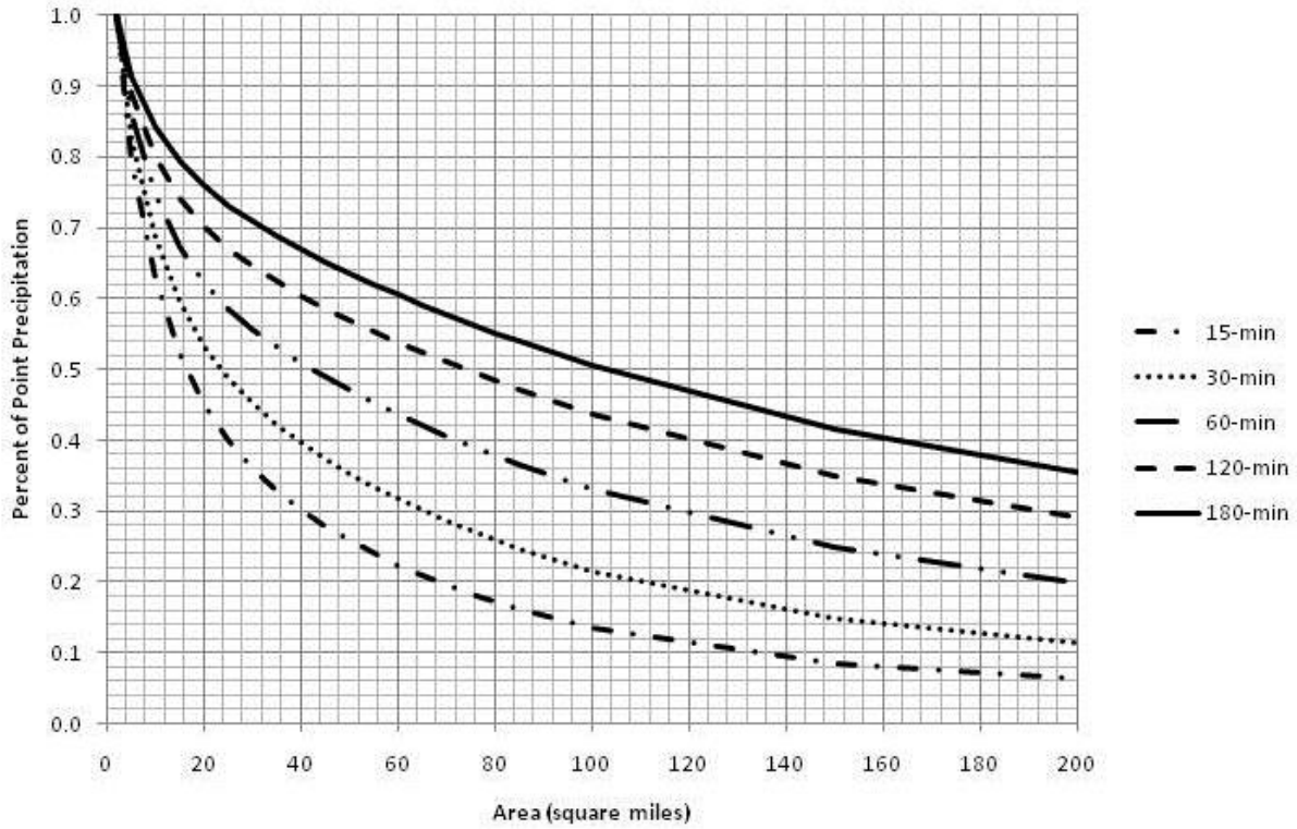
Figure 6-219. Depth-Area-Duration Adjustment Factors for 2-Hour Thunderstorms (Carlton 2011)
