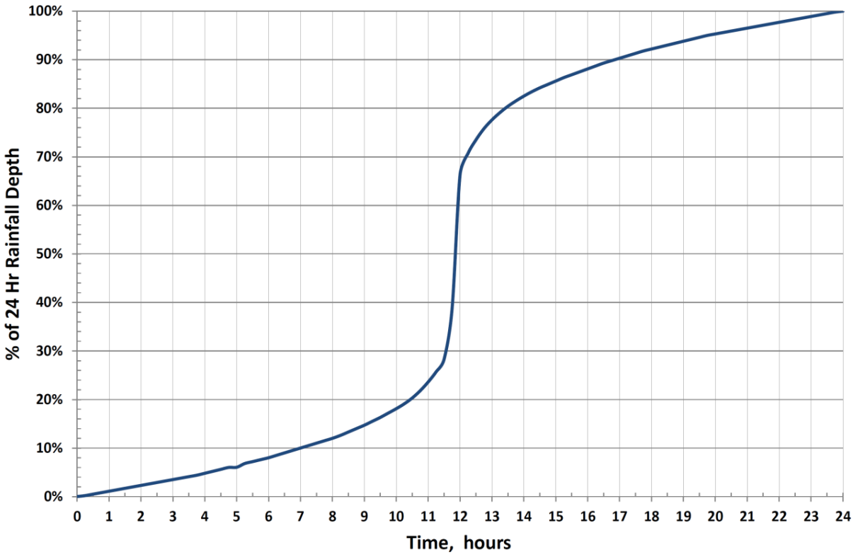
Figure 6-208. NRCS Type II 24-Hour Storm Distribution ( \leq 10 mi 2 )
