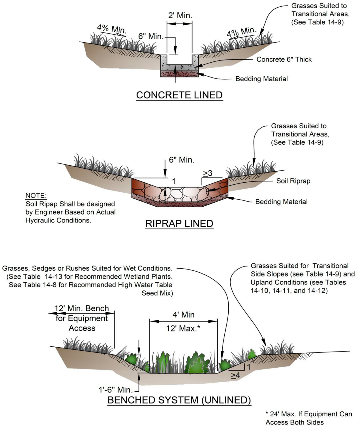
Figure 13-6. Typical Low-flow Channel Details
