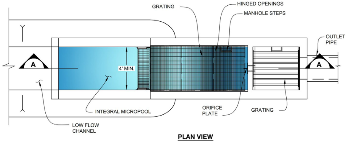
Figure 13-10. Concept for Outlet Structure with Parallel Wingwalls and Flush Bar Grating (Integral Micropool Shown)
