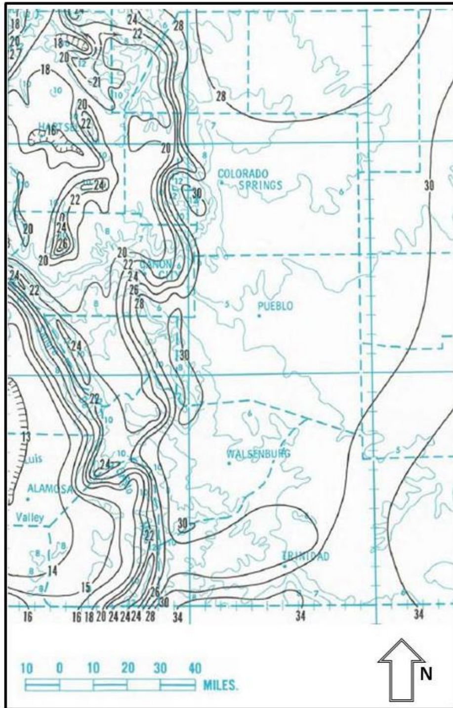
Figure 6-9. 25-Year, 6-Hour Precipitation Tenths of an Inch (NOAA Atlas 2)
