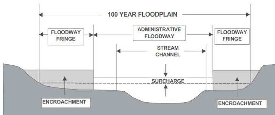
Figure 5-1. Floodplain Schematic
