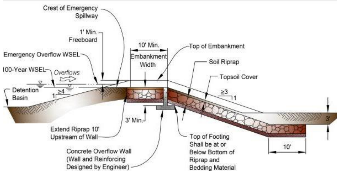
Figure 13-12b. Emergency Spillway Profile at Embankment
