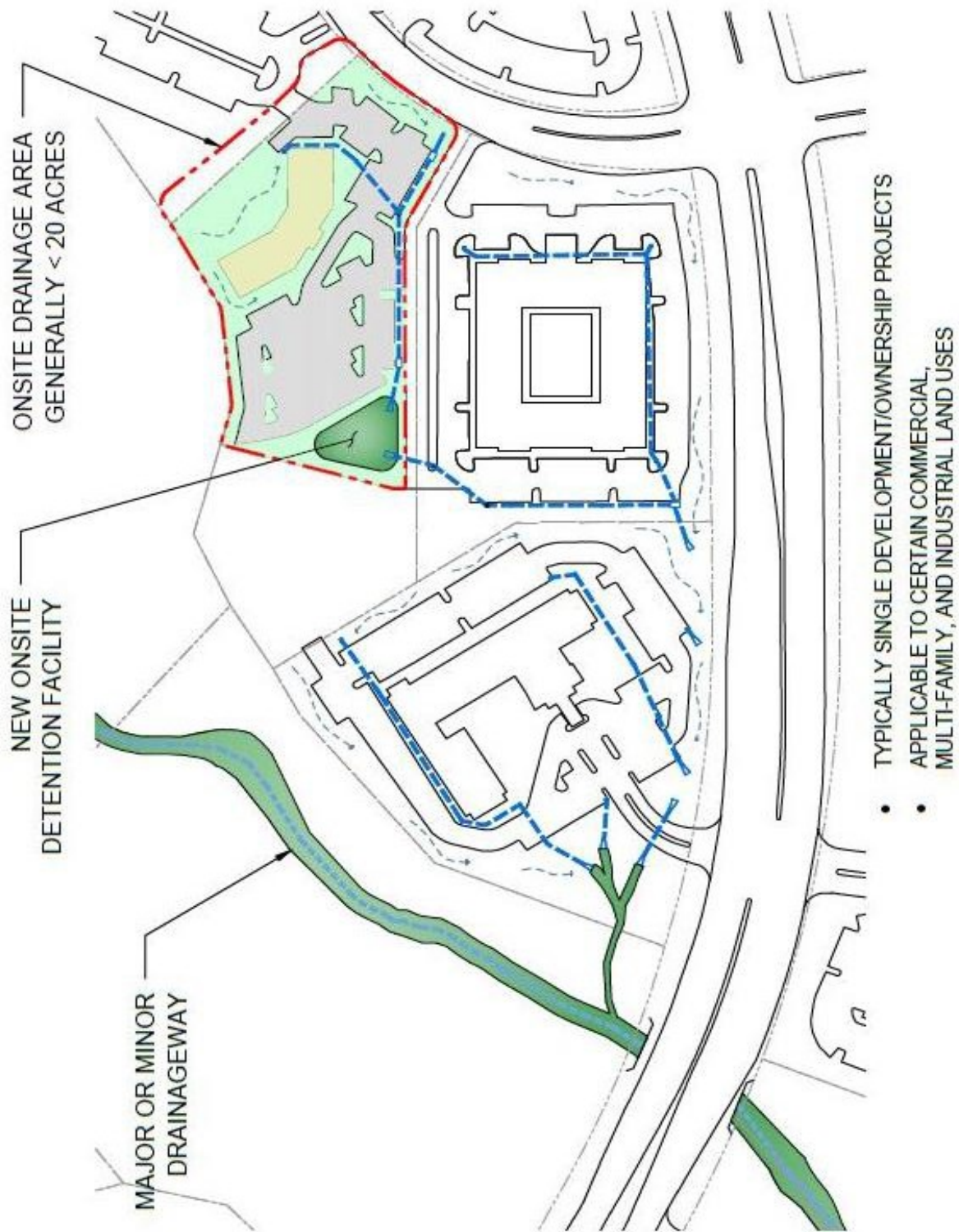
Figure 13-3. On-site Detention Concept
