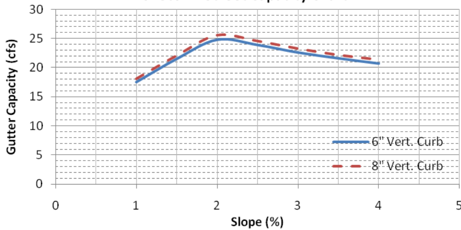
Major Storm Street Capacity Chart
