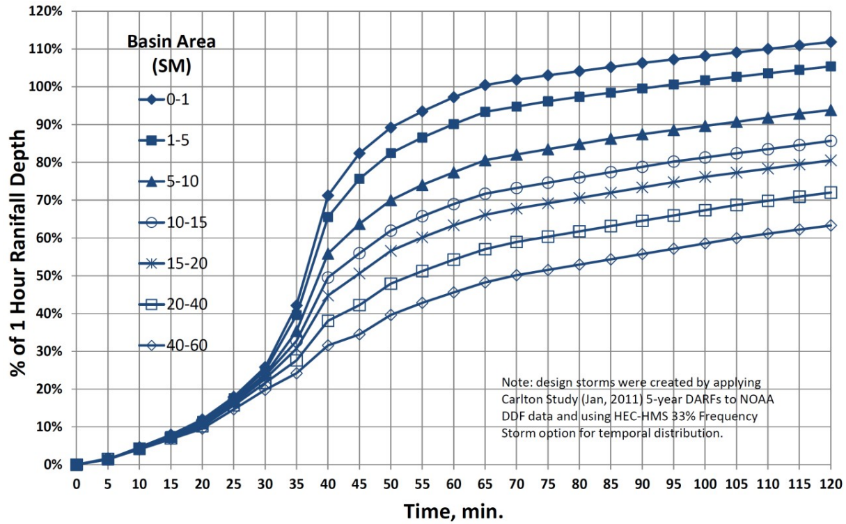
Figure 6-197. 2-Hour Design Storm Distributions By Drainage Basin Area
