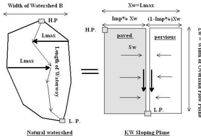
Figure 6-3. SWMM Kinematic Overland Flow Conceptualization of Watershed with Pervious and Impervious Areas
