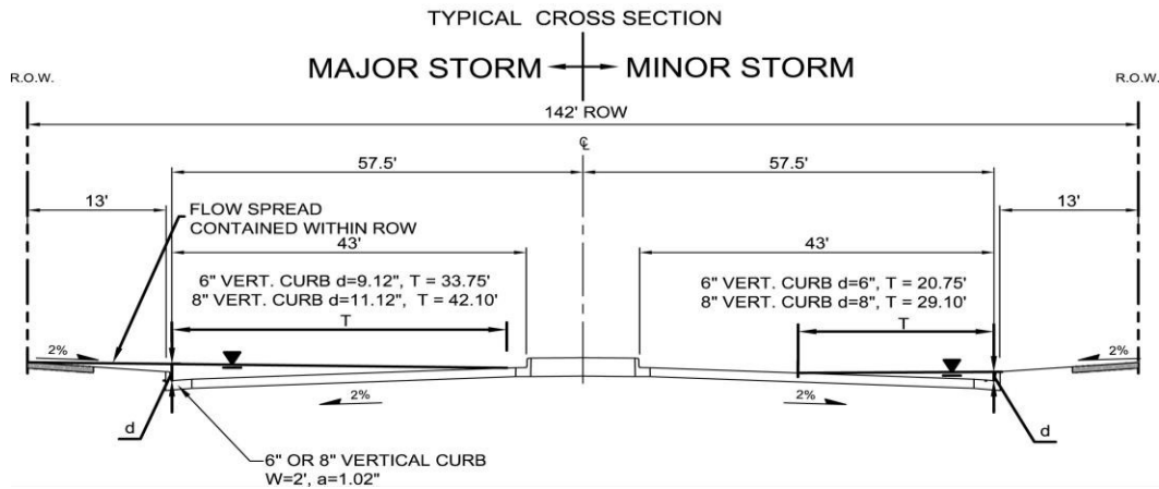
Figure 7-2. Street Capacity Charts Principal Arterial Type II
