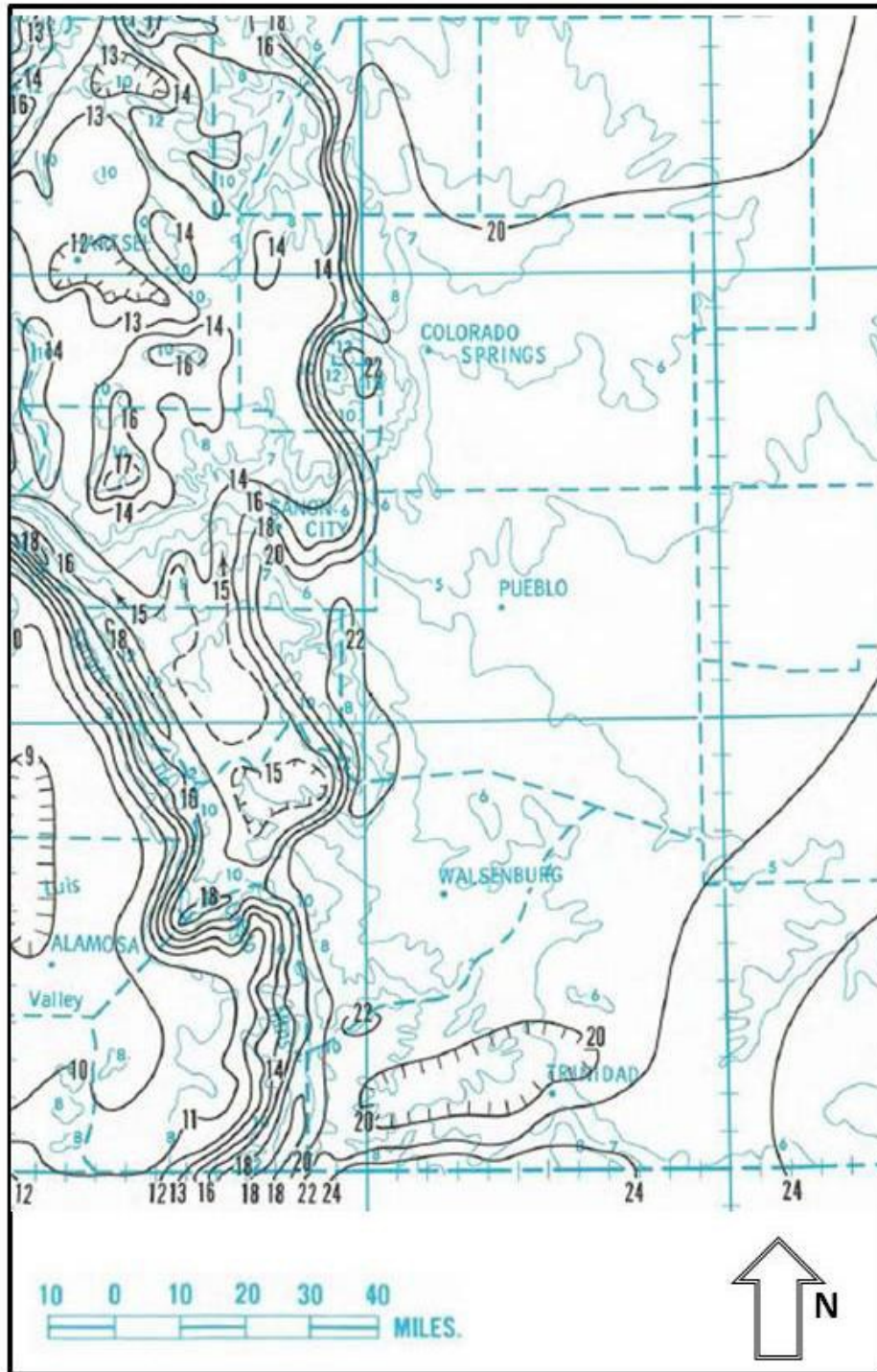
Figure 6-7. 5-Year, 6-Hour Precipitation Tenths of an Inch (NOAA Atlas 2)
