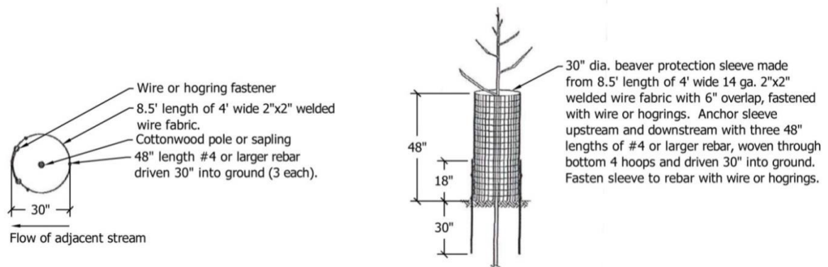
Figure 14-5. Beaver Protection Detail
