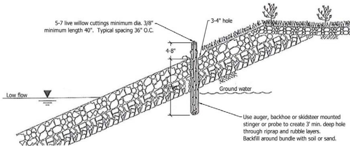
Figure 14-3. Willow Bundling Detail
